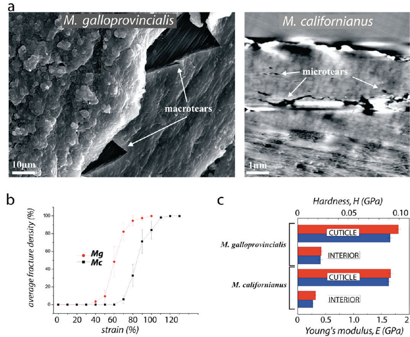
FIGURE 2: Strain tolerance of coatings. (A) At 70% strain, M. galloprovincialis byssal cuticle (left) fails catastrophically, whereas the cuticle of M. californianus (right) exhibits only microtears. (B) Cuticle macrotear formation during thread extension can be monitored by microscopic inspection. M. californianus cuticle has a higher strain capacity compared to that of M. galloprovincialis as demonstrated by its lower tear tendency or fracture density at any given strain (100% average fracture density represents whole thread failure). (C) Nanoindentational hardness and modulus of hydrated thread cuticle and interior of both mussel species ( N = 13 ; brackets are standard deviations).
