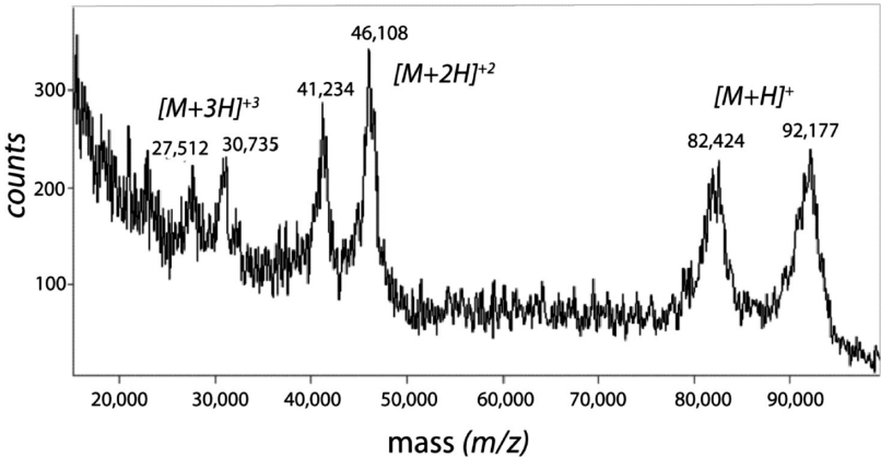
FIGURE 3: MALDI-TOF mass spectrum of purified mcfp-1. Peak clusters from right to left are singly, doubly, and triply protonated ions. Operating parameters were delayed extraction (200 ns) in positive ion mode with accelerating voltage of 25000 V, grid voltage at 93%, and guide wire voltage at 0.1%. Spectrum represents the average of 254 scans.
